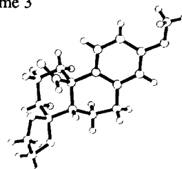
Figure 1. ORTEP diagram of 11a
